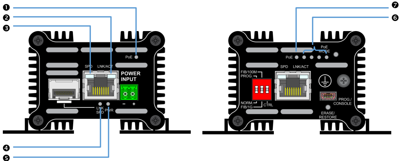
FIGURE 5: PORT/LED
