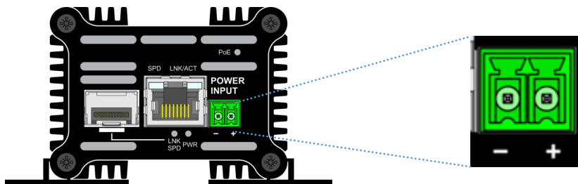
Front Panel
