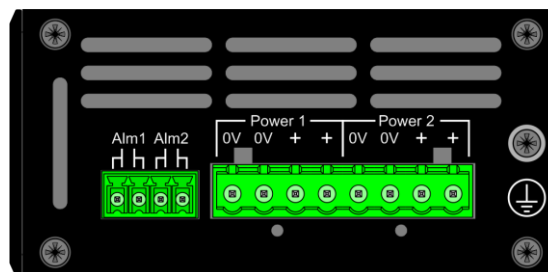
FIGURE 5: ALARM OUTPUTS
