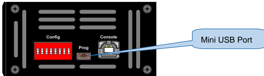
FIGURE 9: USB CONNECTOR
