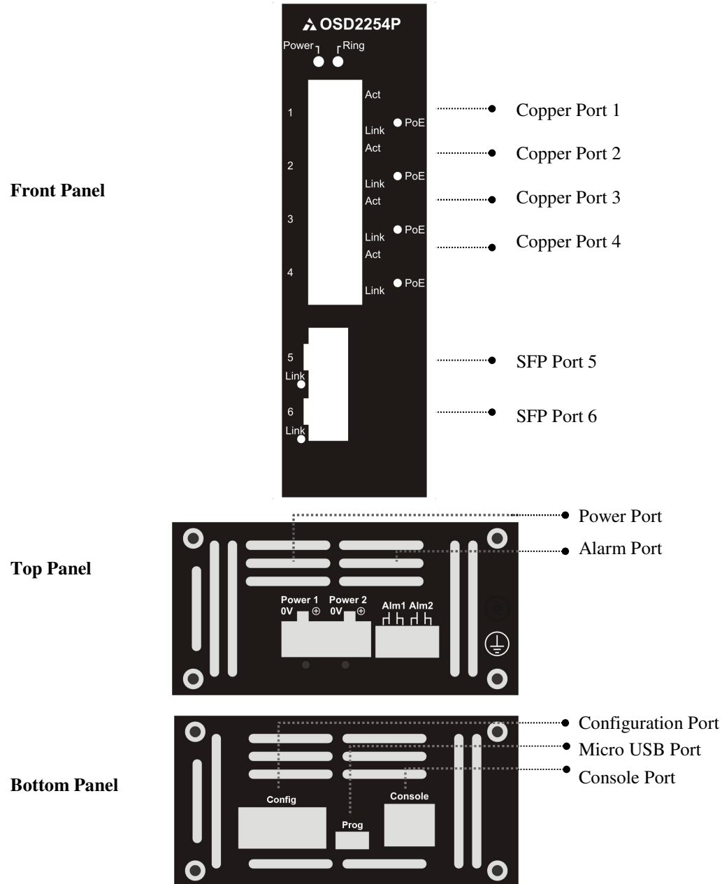
FIGURE 2: OSD2254P PORT ALLOCATION
