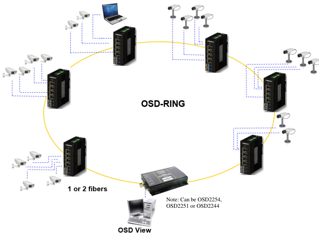
FIGURE 1: OSD2254P TYPICAL RING CONFIGURATION
