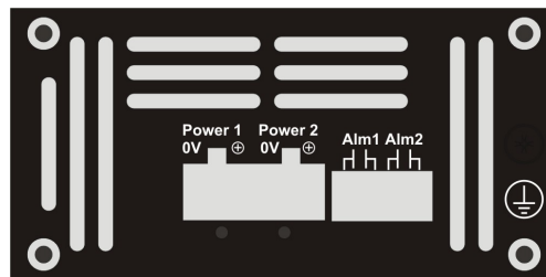
FIGURE 4: OSD2254P POWER SUPPLY CONNECTIONS
