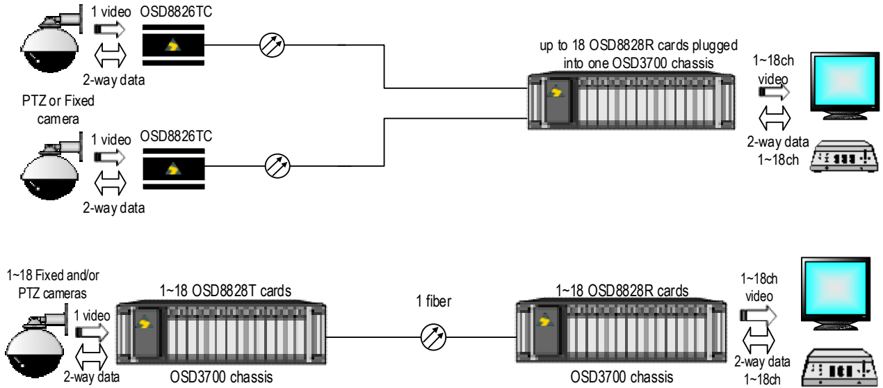
FIGURE 1: OSD8828 TYPICAL CONFIGURATIONS
