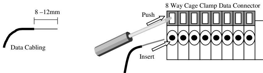
FIGURE 4: DATA CABLING CONNECTIONS
