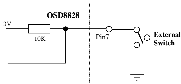
FIGURE 6: OSD8828T CONTACT CLOSURE INPUT
