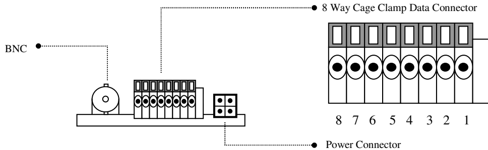
FIGURE 3: DATA CONNECTOR PINOUTS
