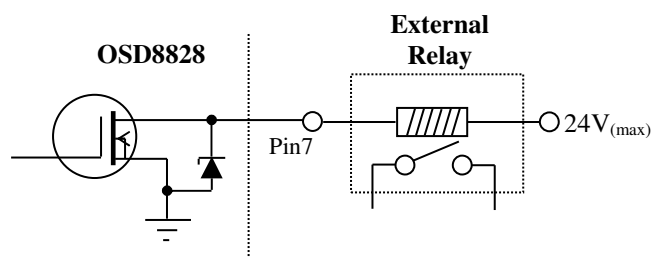
FIGURE 7: OSD8828R CONTACT CLOSURE OUTPUT
