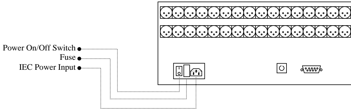
FIGURE 5: OSD725 POWER SUPPLY CONNECTIONS
